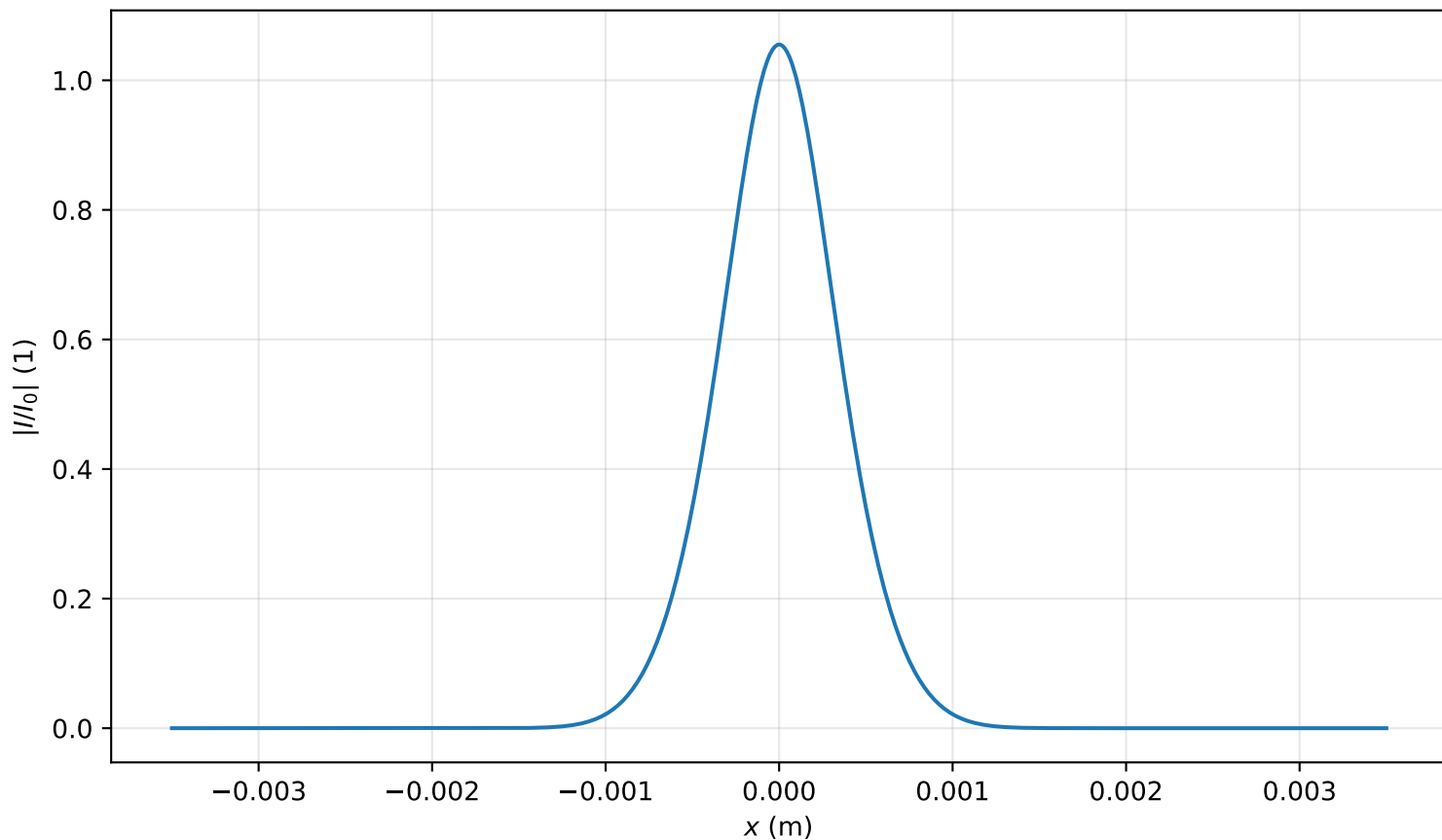
Intensity profile I(x, y = 0, z = 0.637m)/I_0 , P_{in}=0.5P_{cr} , artificial time
